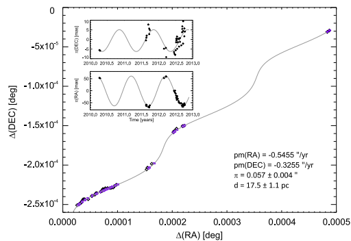
Fig. 2. Parallax of VVV BD001, the distance was measured based on relative astrometry with a precision of a few mas ( \pi=0.057 \pm 0.004'' ), as more data become available, increasing the time baseline and number of observations, the astrometric precision will improve to become close to 1 mas. Explained in Beamin et al. (2013)
