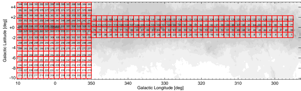
Fig. 1. VVV Survey area and tile numbering. The tile names start with “b” for bulge and “d” for disk tiles, followed by the numbering as shown in the figure. (Credit: Saito et al. (2012) A&A 537, A107, reproduced with permission ©ESO.)
